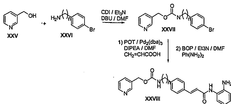
Scheme 4
